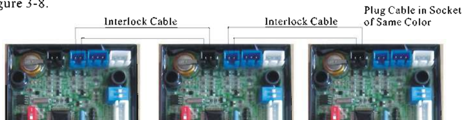
Figure 3-8 Network System Wiring with Interlock Cable
