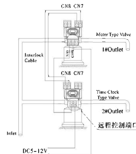
Figure3-11 Series system
