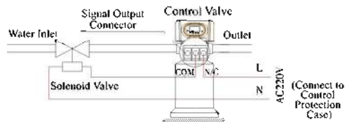
Figure 3-2 Wiring of Solenoid Valve on Inlet
