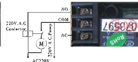
Figure 3-7 Wiring of Booster pump on Inlet
